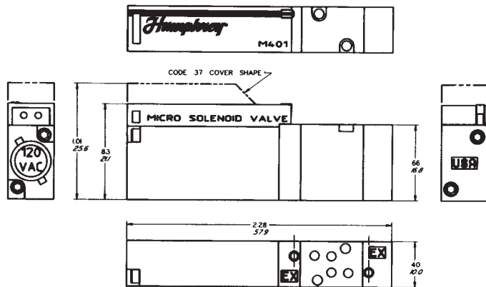
401/402 Air Flow To Atmosphere
